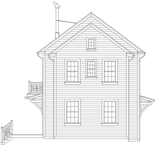
01 SOUTH ELEVATION A.3 1/4" = 1'-0" SCALE
