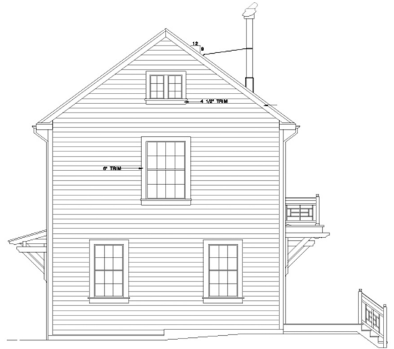
NORTH ELEVATION
